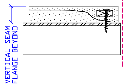
V VERTICAL SECTION
