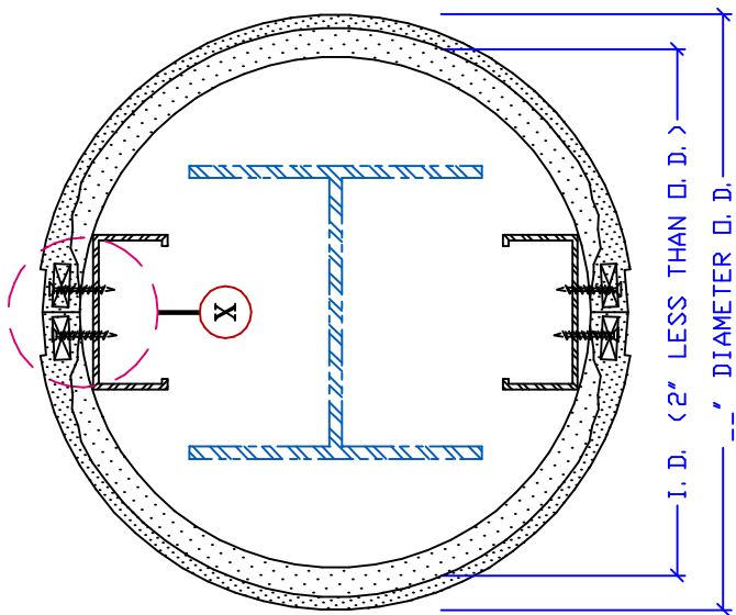
P PLAN VIEW
